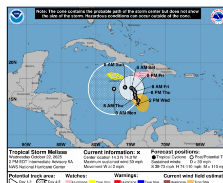
The forecasted track of Hurricane Melissa as of 22 October
